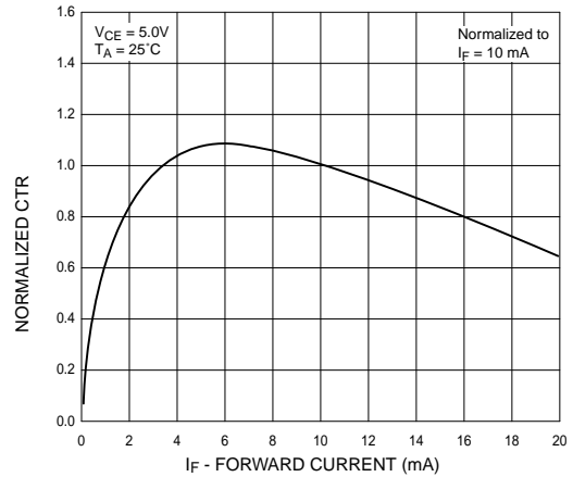
Fig.2 Normalized CTR vs. Forward Current (White Package)
