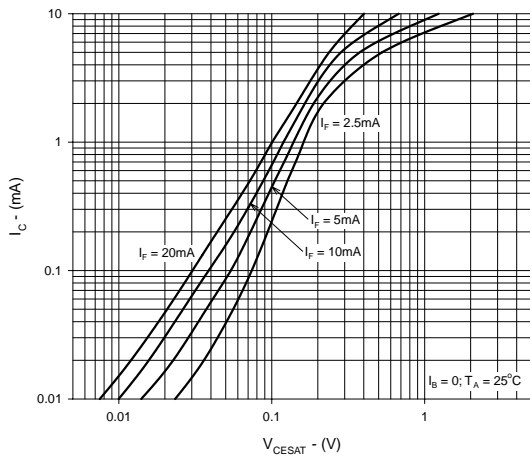
Fig. 17 Collector Current vs. Collector-Emitter Saturation Voltage
