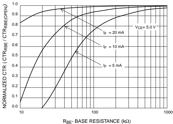
Fig.5 CTR vs. RBE (Unsaturated) (Black Package)
